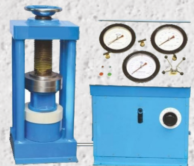
Compression Testing Machine Electrical
