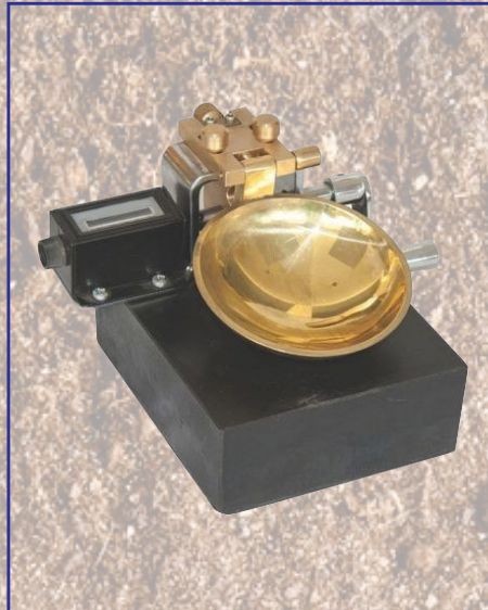
Liquid Limit Device with Counter
