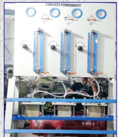
Concrete Permeability Test Apparatus
