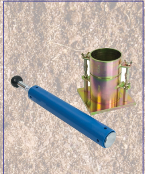
Standard Compaction Test
